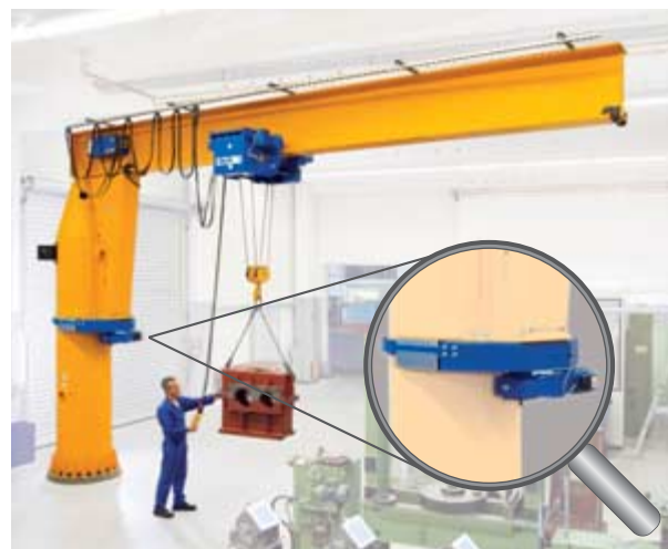
Powered slewing (Fig. 2)
